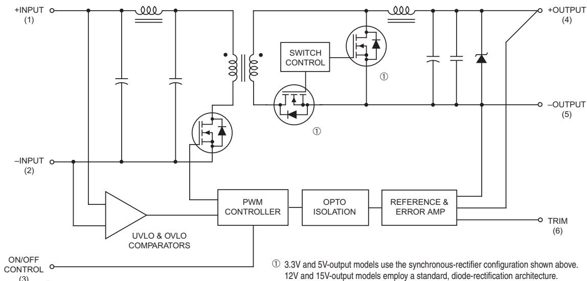
Figure 1. Simplified Schematic
